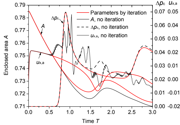
Figure 8: Stability comparison between the coupling schemes with and without iterations. The history of the enclosed area, pressure at center point c and x-velocity component at point a for the membrane relaxation case. k_s=0.05 , \nu=0.001 .
