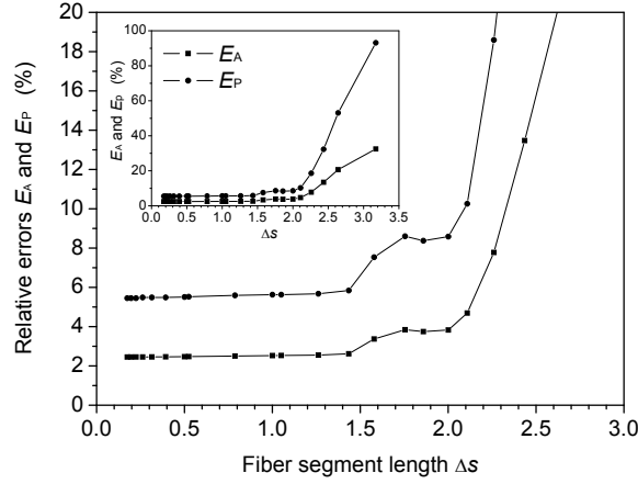
Figure 20: Error dependence on the fiber segment length for the membrane relaxation case.
