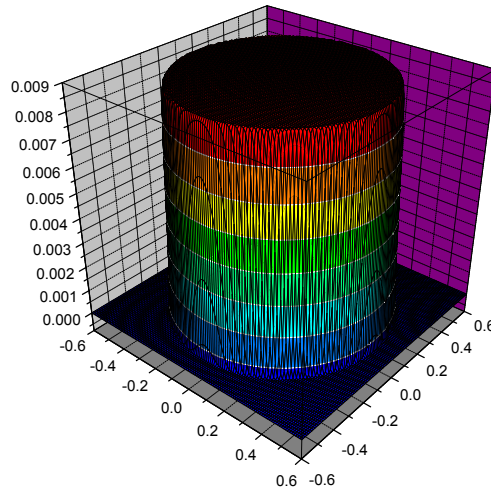
Figure 5: Wire-surface of the pressure value of the relaxing membrane at near equilibrium state T=1000 . They are from the scheme with \phi_4^{\text{IB}} and 5 iterations per cycle, and the parameters are N=200 , n_b=1200 , r_i=0.5 , k_s=0.02 , l_r=0.8l_i , \nu=0.001 .
