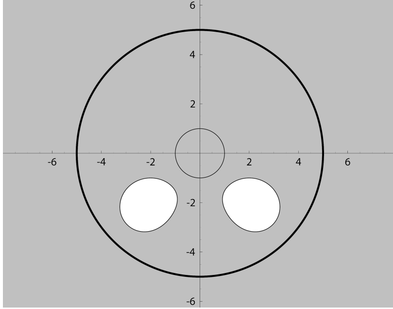
FIGURE 3. The set \varphi^{-1}(\mathbb{D}) for \varphi(z) = (z^2 + 2iz + 3)/(2z^2 + 8iz - 14) , along with \partial\mathbb{D} and \mathcal{C}_R for R = 5 .
